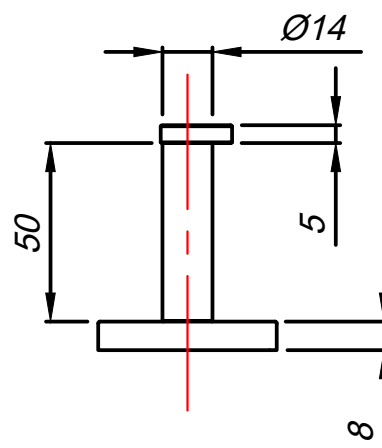
Mounting Plate
