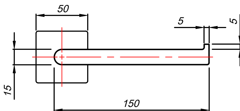
Mounting Plate
